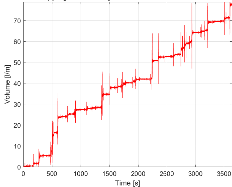
Overtopping Time History - Test: H03C1R1WO Data: 20-06-19
